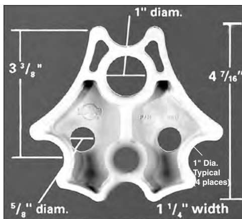
5060150B – (1-1/4" width)
