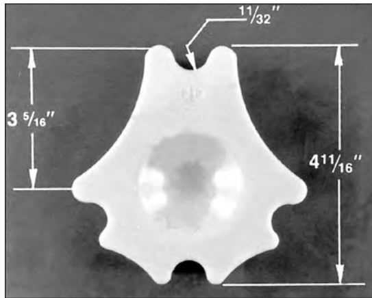
5060100 – Front View
